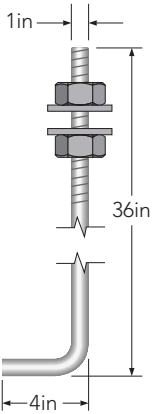
A3 Anchor Bolt Suit for 30ft
