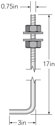
A1 Anchor Bolt Suit for 10ft, 15ft, 20ft
