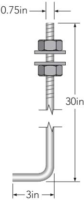
A2 Anchor Bolt Suit for 25ft
